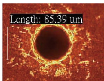
(Brown-oxide Copper direct drill Φ85 μm)
